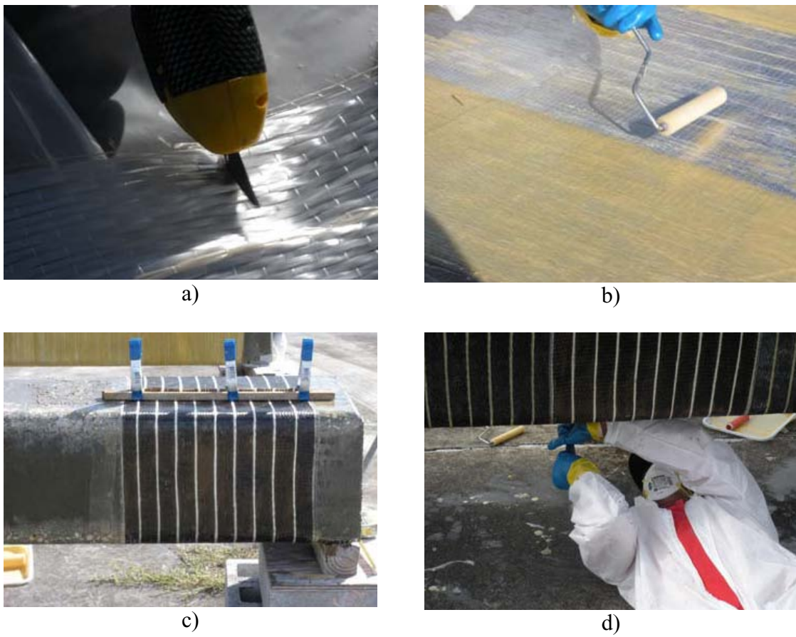
Fig. A - 5: Wrapping of the column specimens: cutting of the fiber sheet (a); installation of the fiber sheet (b-d).
