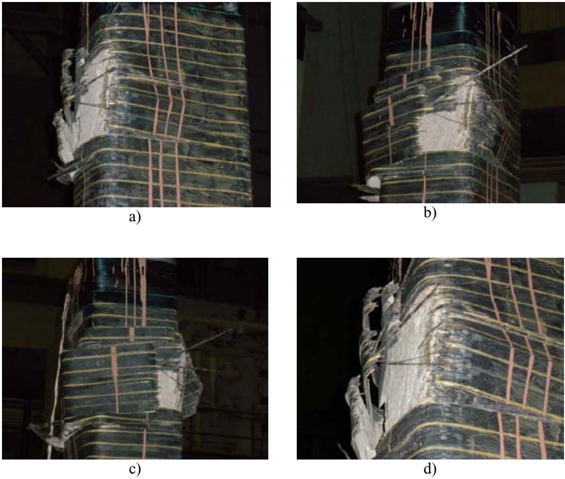
Fig. A - 33: Failure of Specimen R-0.5-8H (a-d).
