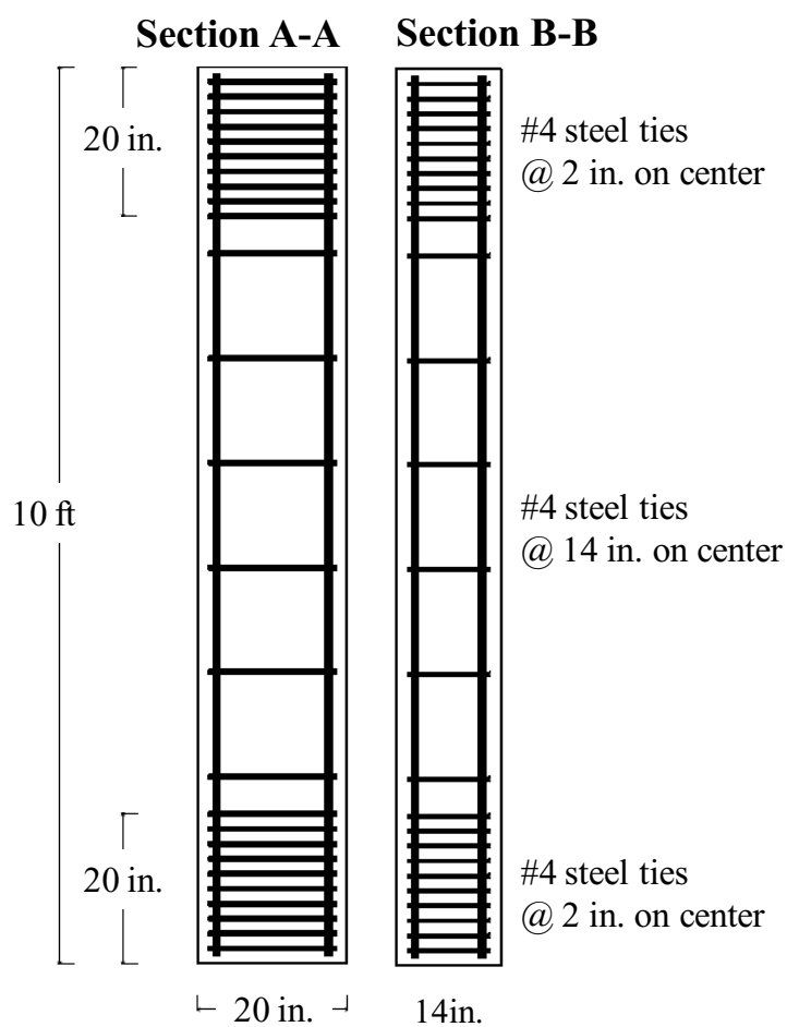
Fig. 11: Reinforcement layout for series R-0.5.
