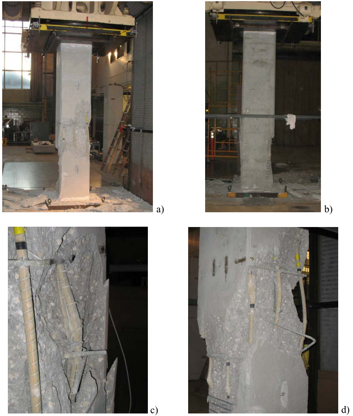
Fig. A - 18: Failure of Specimen A-12 (a-d).
