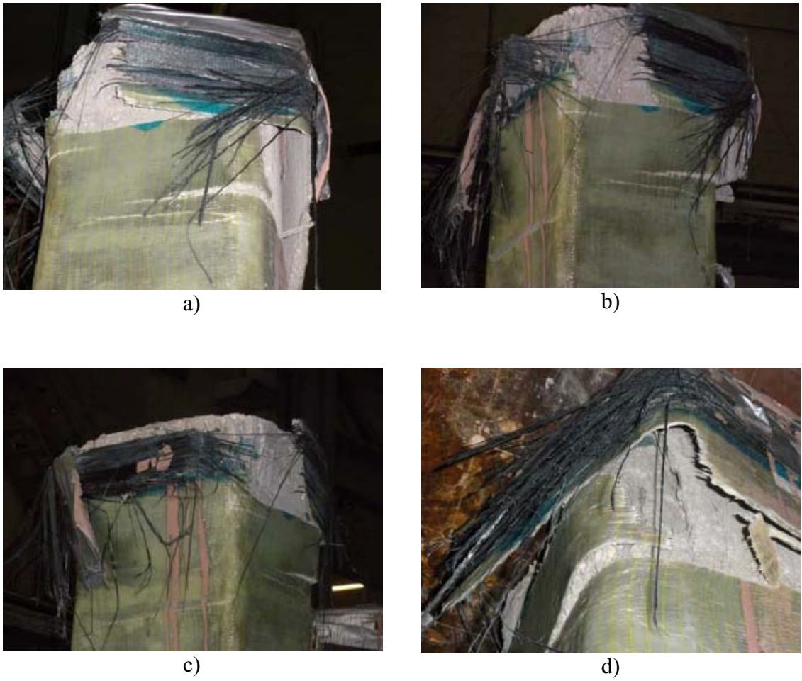
Fig. A - 31: Failure of Specimen R-0.5-2GB (a-d).
