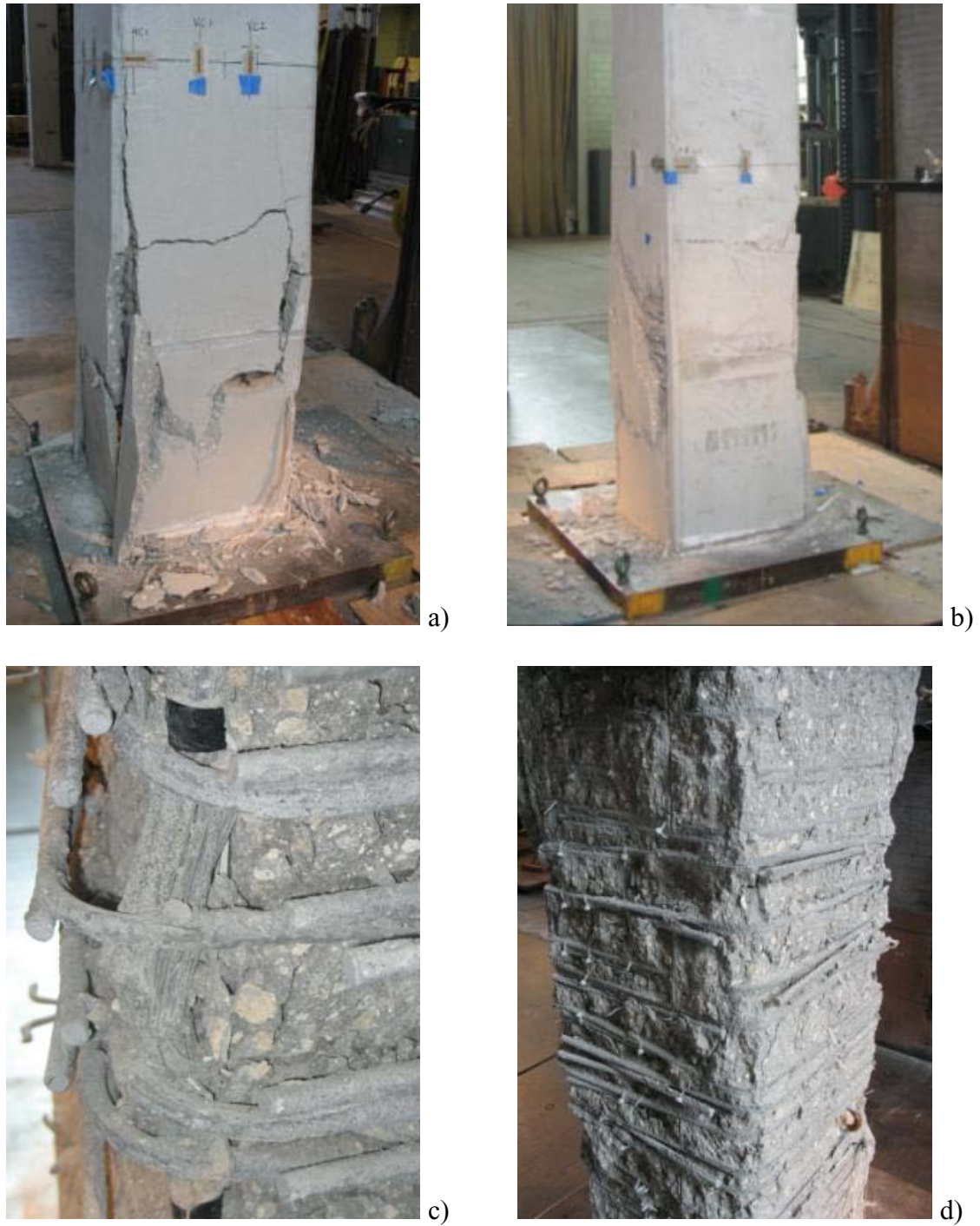
Fig. A - 21: Failure of Specimen B-3 (a-d).
