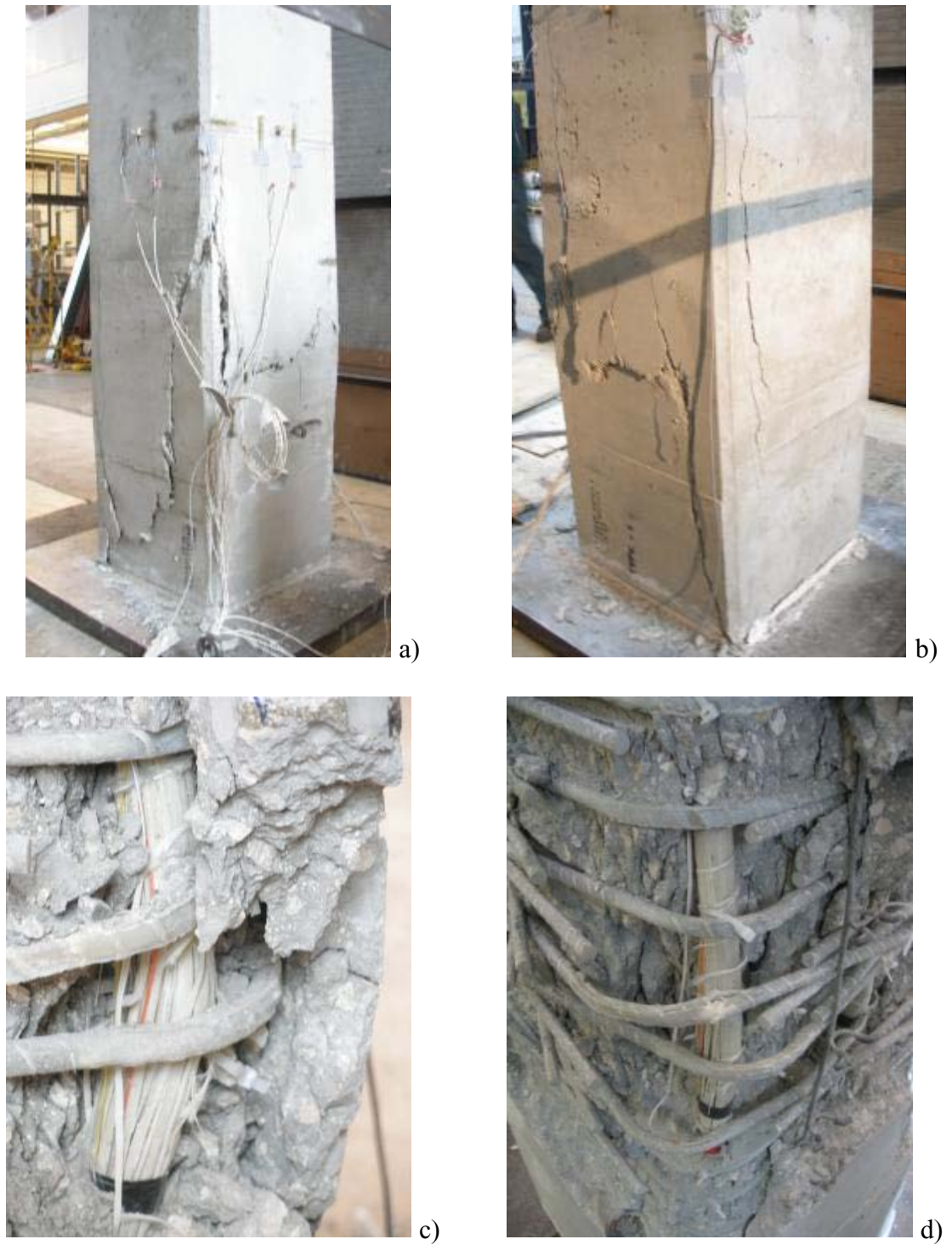
Fig. A - 20: Failure of Specimen A-3 (a-d).
