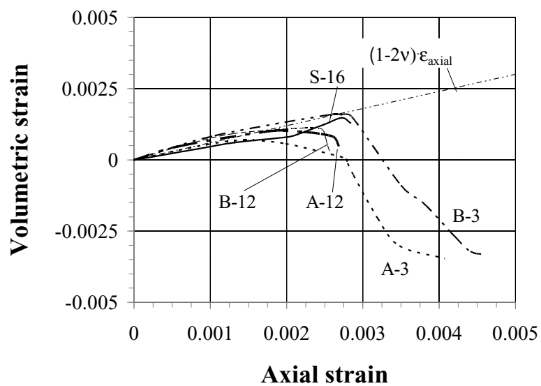
Fig. 7: Volumetric strain-axial strain.
